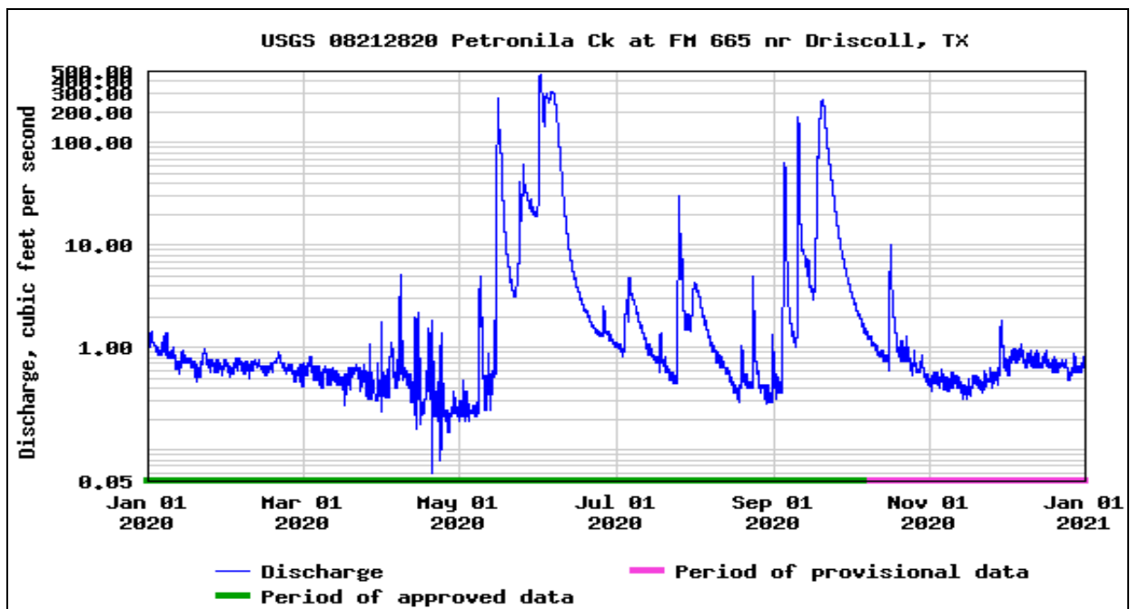
Figure 10. USGS sourced streamflow at Petronila Creek Above Tidal at FM 665
