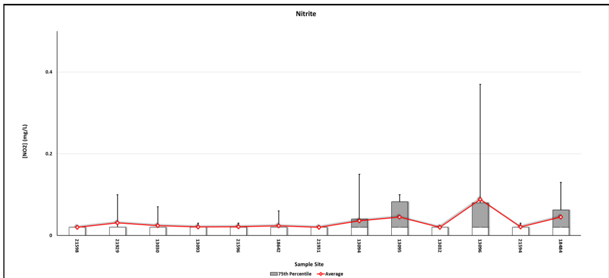
Figure 20. Annual mean nitrite concentrations at tributary stations
