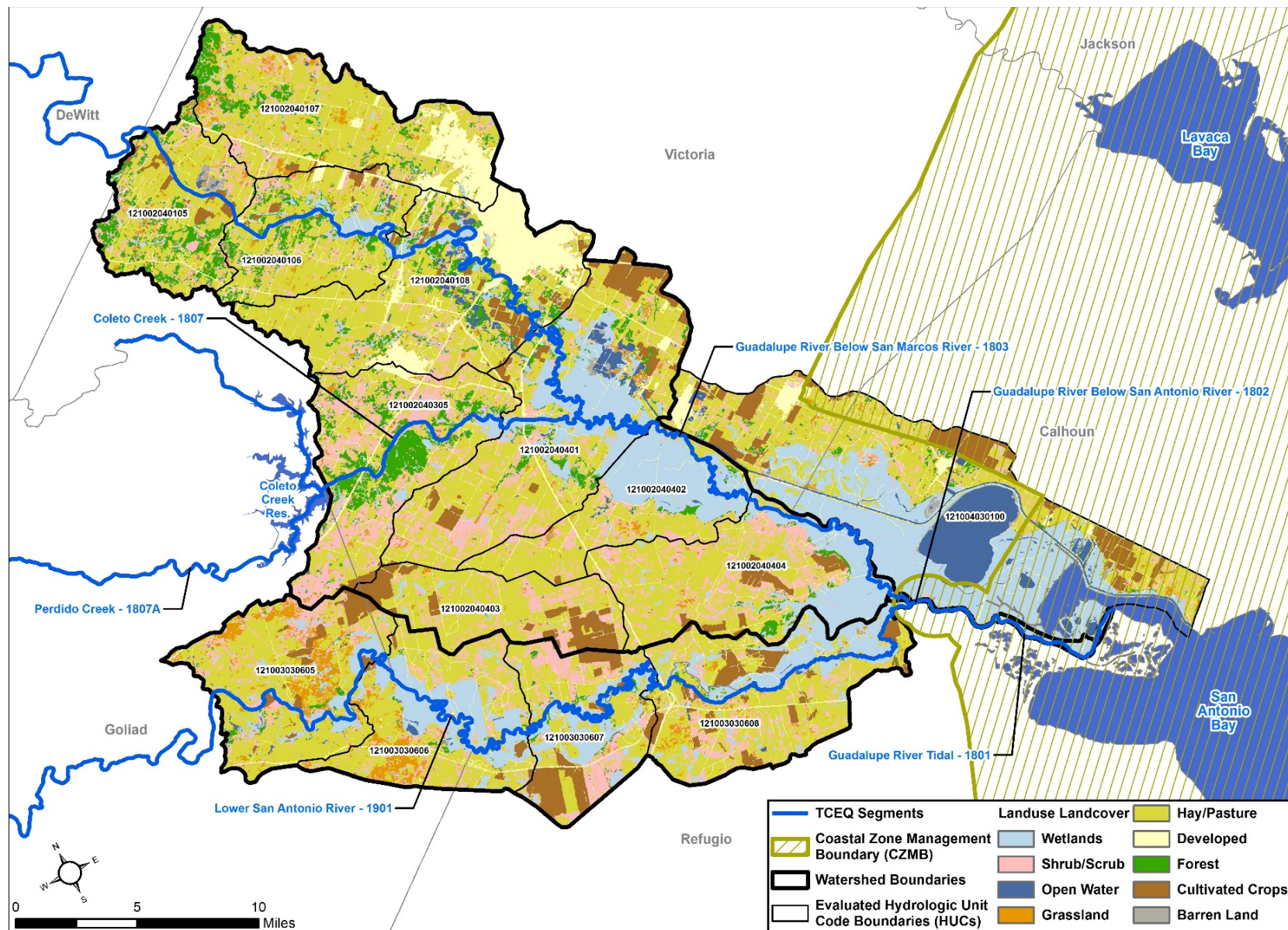
Figure 3-2 Lower Guadalupe River Watershed Land Use and Land Cover
