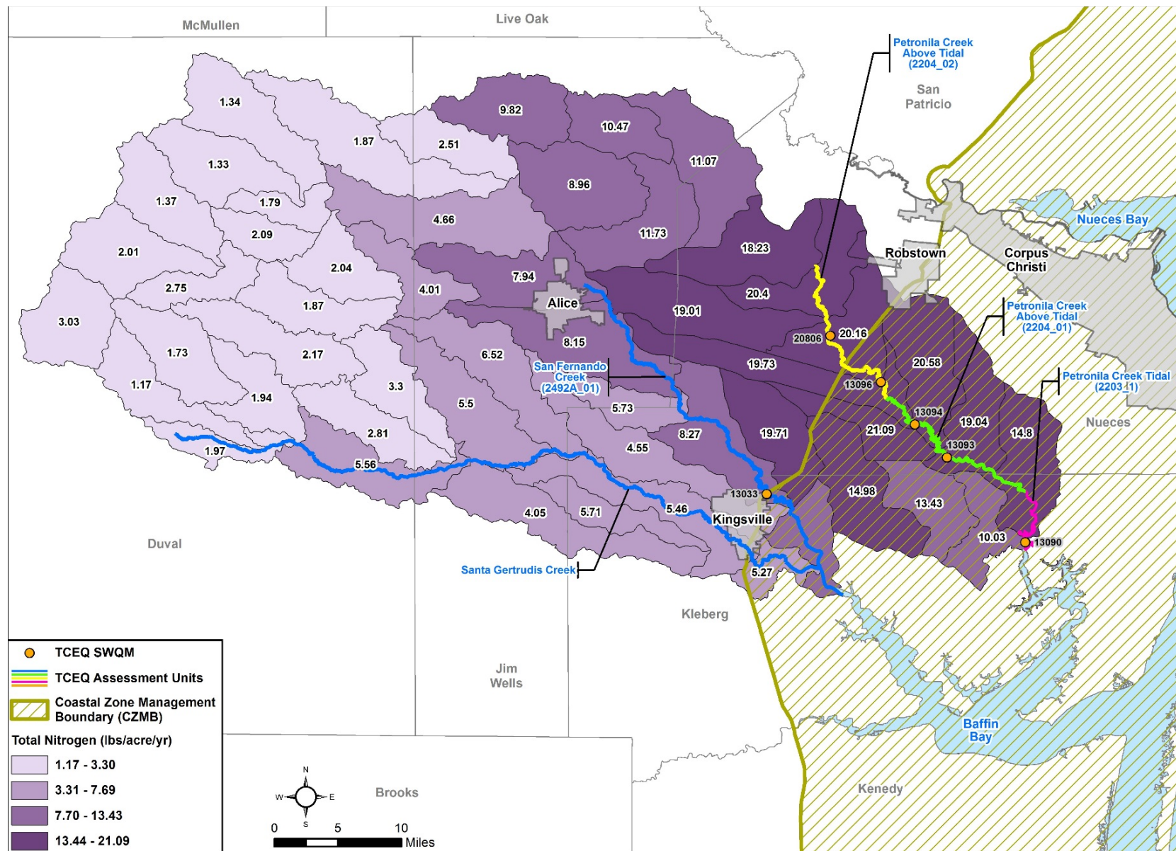
Figure 3-10 San Fernando Creek and Petronila Creek 12-Digit HUCs - Nitrogen Load Estimates
