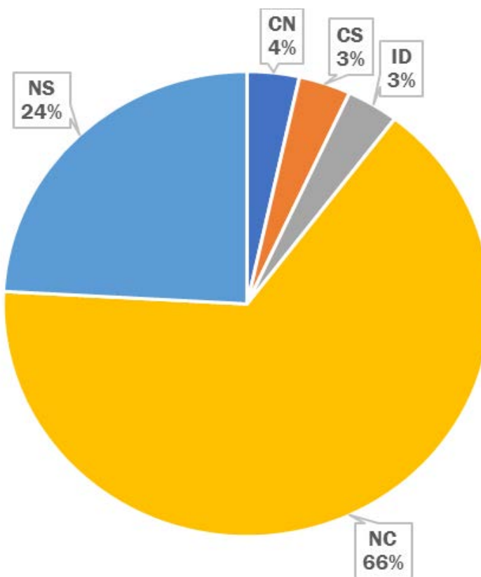
Figure 2-4 2014 Dissolved Oxygen ILOS for Nutrient-Impacted Coastal Waters (n=58)
