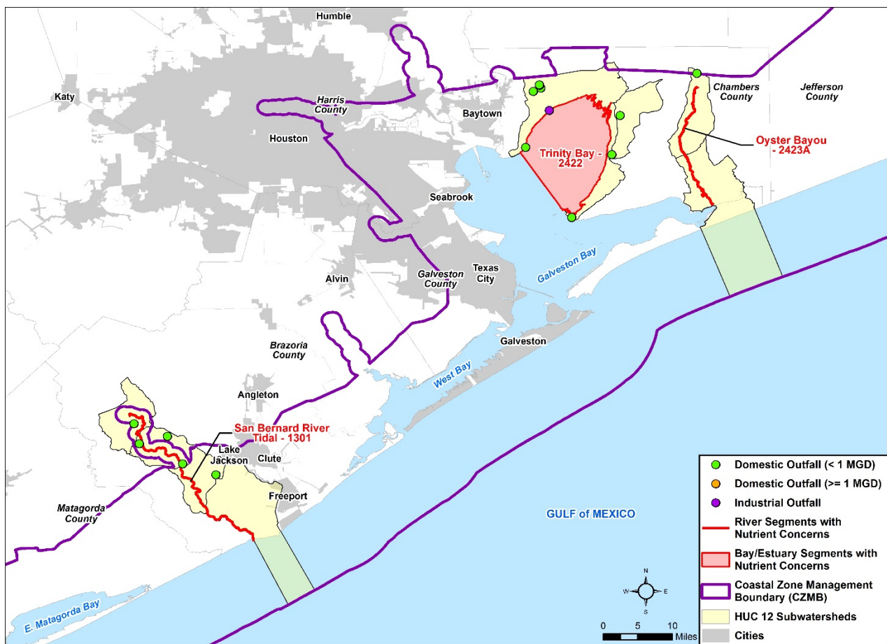
Figure 2-6 Non-urban, Nutrient-impacted Watersheds within the Coastal Zone Boundary (Northern Coast)
