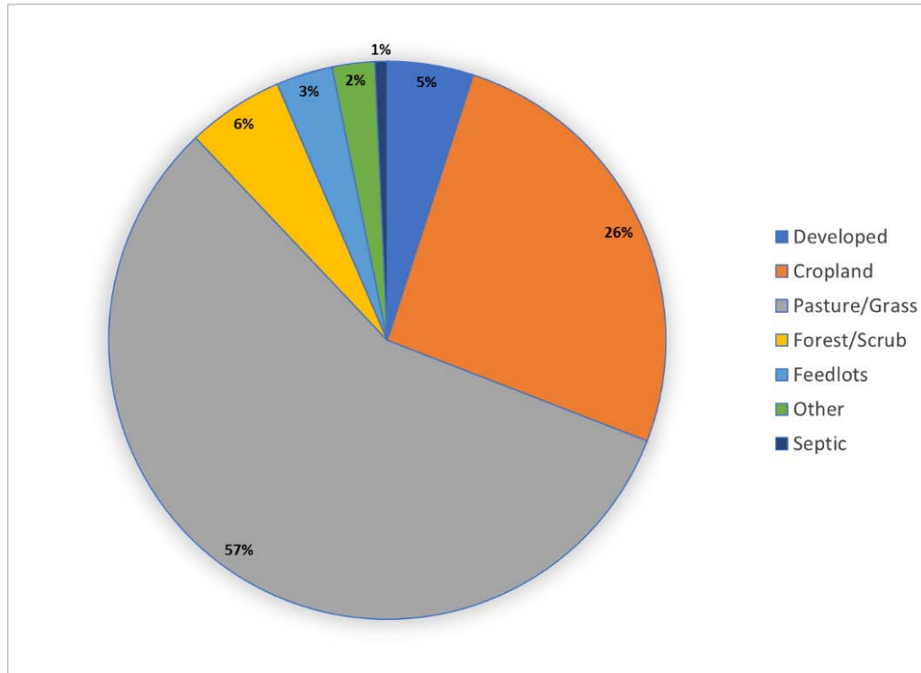
Nitrogen Loads – Lower Guadalupe River Watershed
