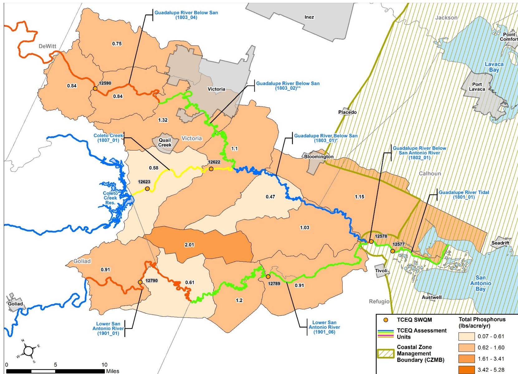
Figure 3-8 Lower Guadalupe River 12-Digit HUCs - Phosphorus Load Estimates
