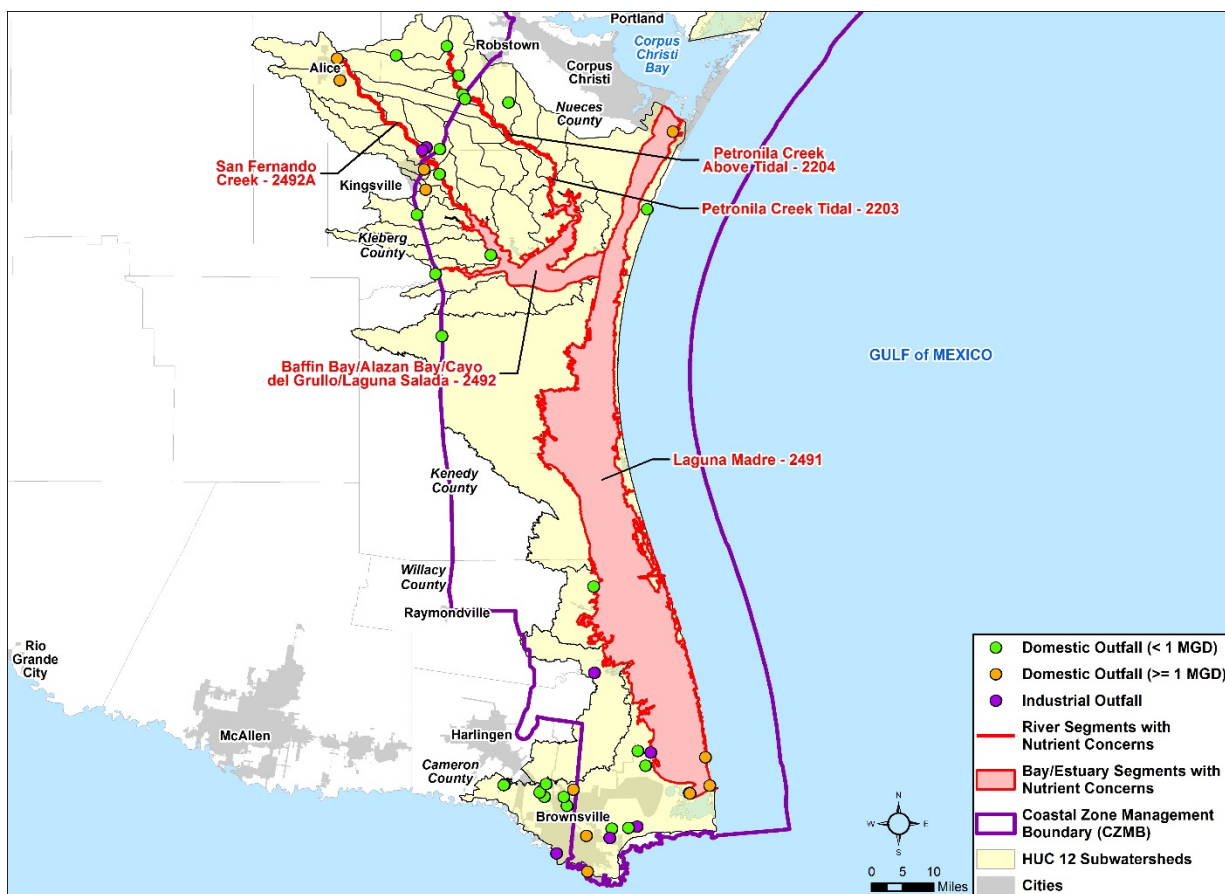
Figure 2-8 Non-urban, Nutrient-impacted Watersheds within the Coastal Zone Boundary (Southern Coast)
