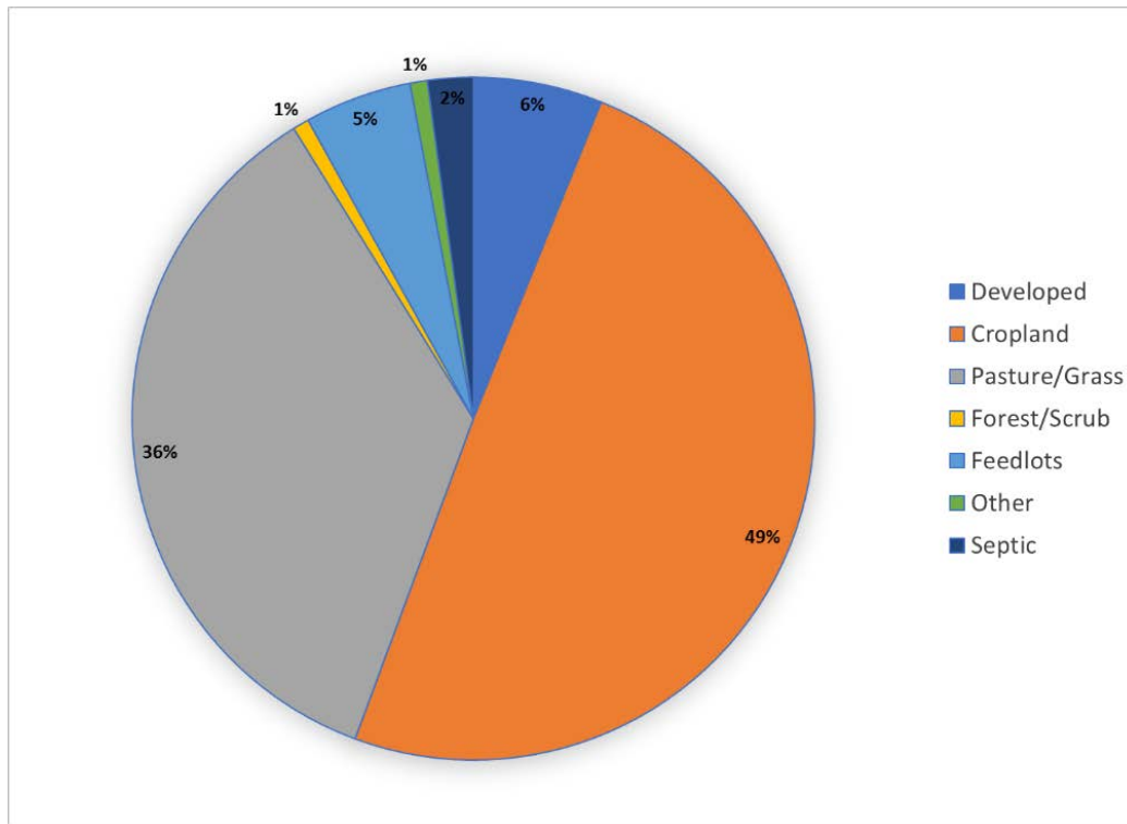
Phosphorus Loads – Lower Guadalupe River Watershed
