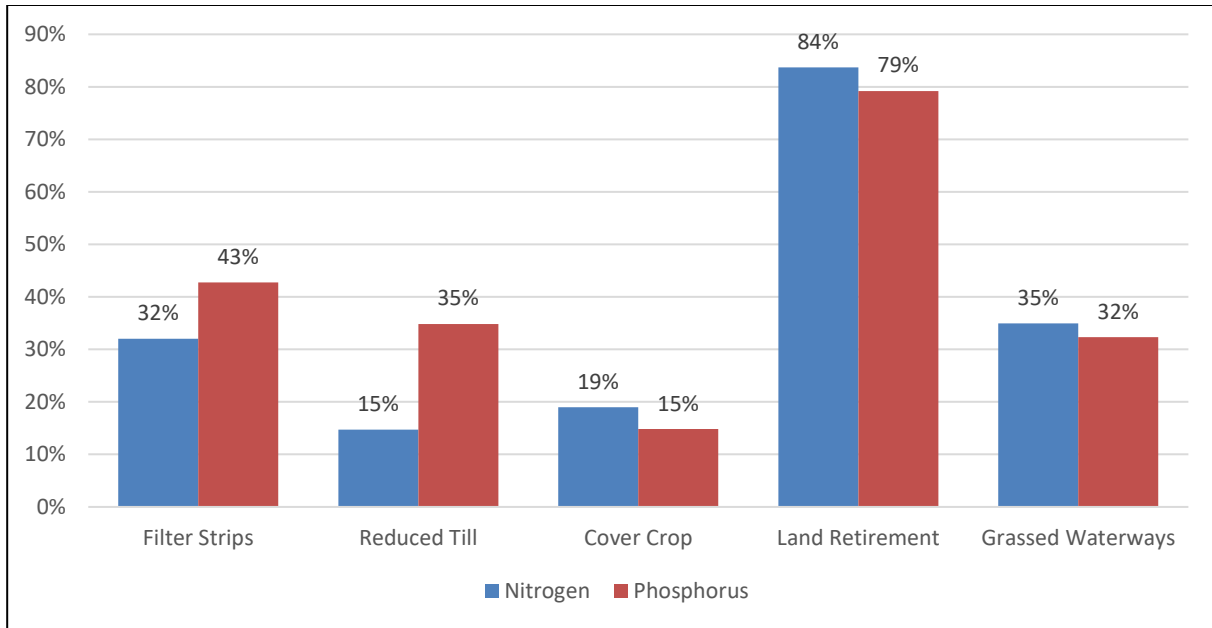
Figure 4-3 BMP Nutrient Load Reduction Potential (Group 1)
