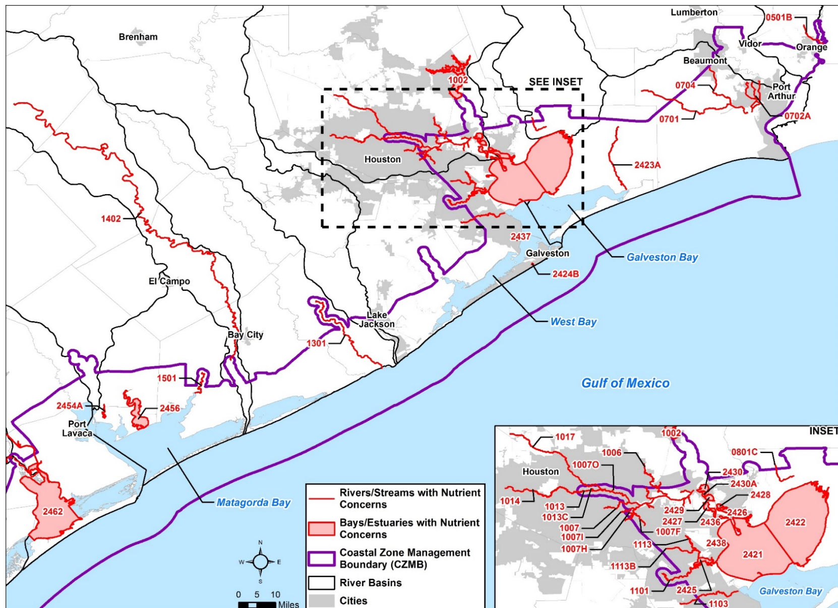
Figure 2-2 Texas Upper Coast Segments with Significant Nutrient Concerns (n=58)
