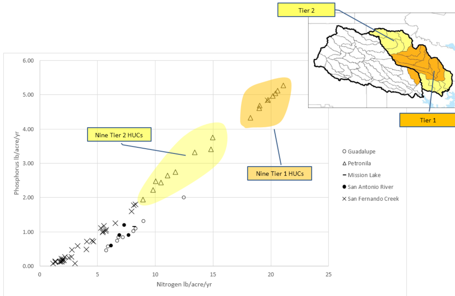
Figure ES-4 Phosphorus/Nitrogen Scatterplot of all HUCs
