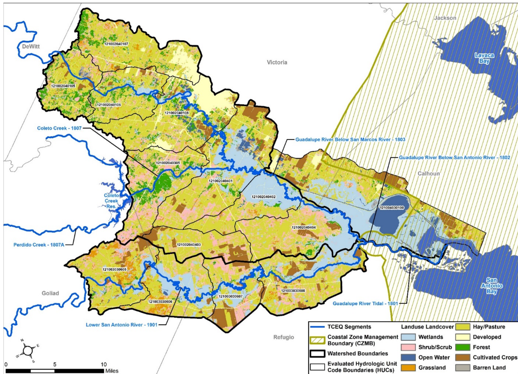
Figure ES-2 Lower Guadalupe River Watershed Land Use and Land Cover
