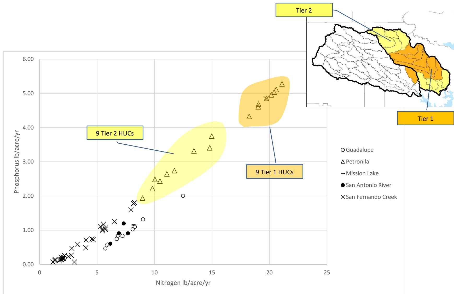
Figure 3-13 Phosphorus/Nitrogen Scatterplot of all HUCs
