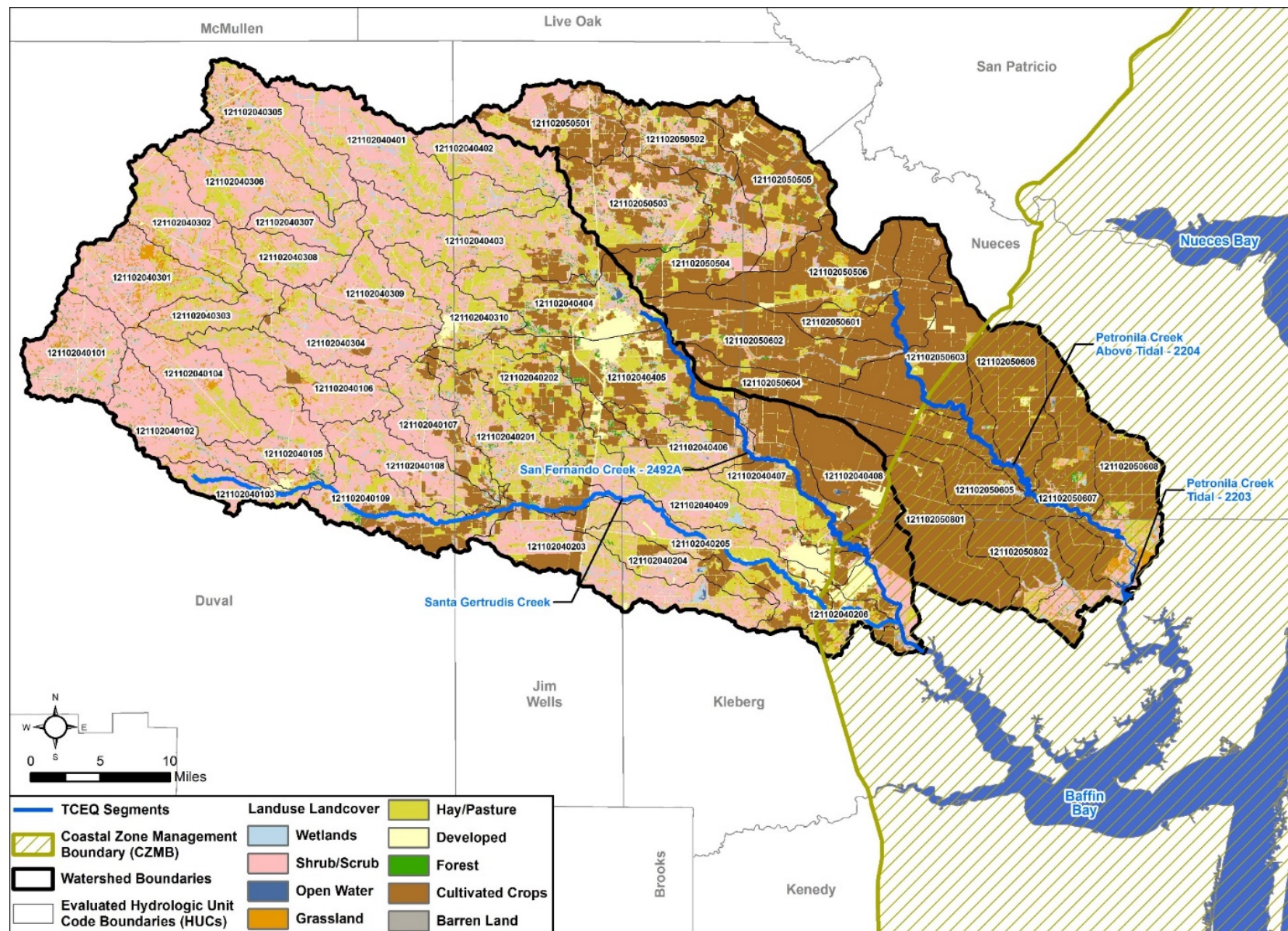
Figure ES-3 San Fernando Creek and Petronila Creek Watersheds Land Use and Land Cover
