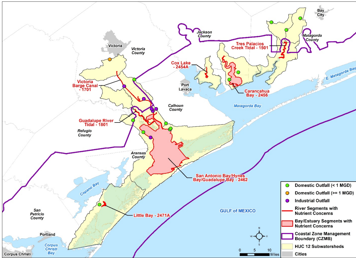
Figure 2-7 Non-urban, Nutrient-impacted Watersheds within the Coastal Zone Boundary (Central Coast)
